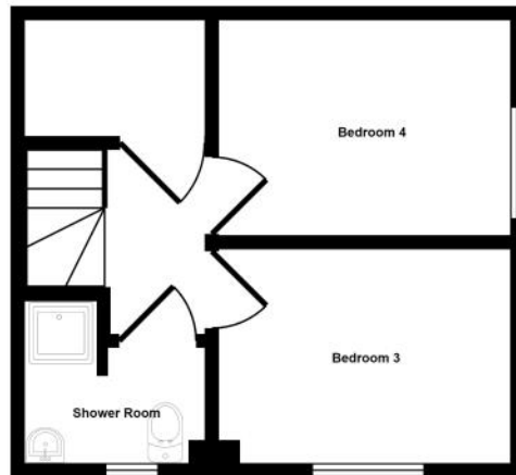
Lower Ground Floor Approx 24 sq m / 262 sq ft
