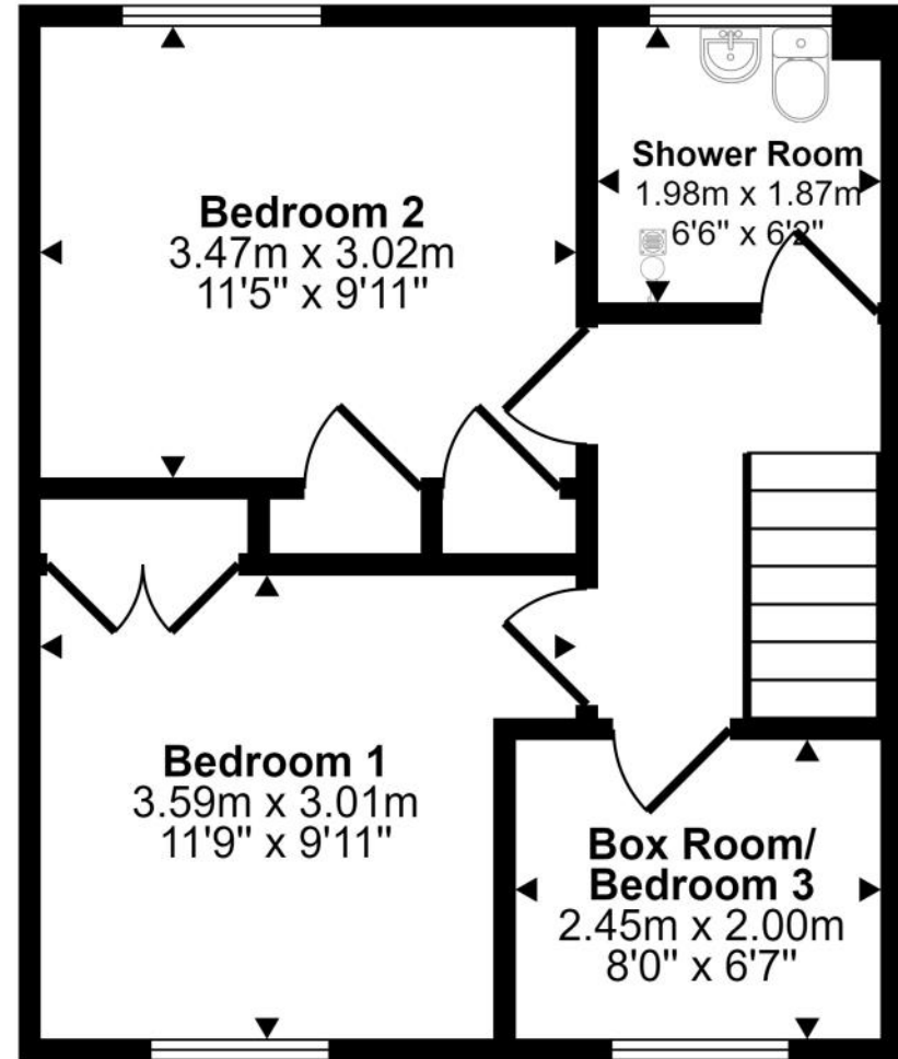
First Floor Approx 38 sq m / 405 sq ft
