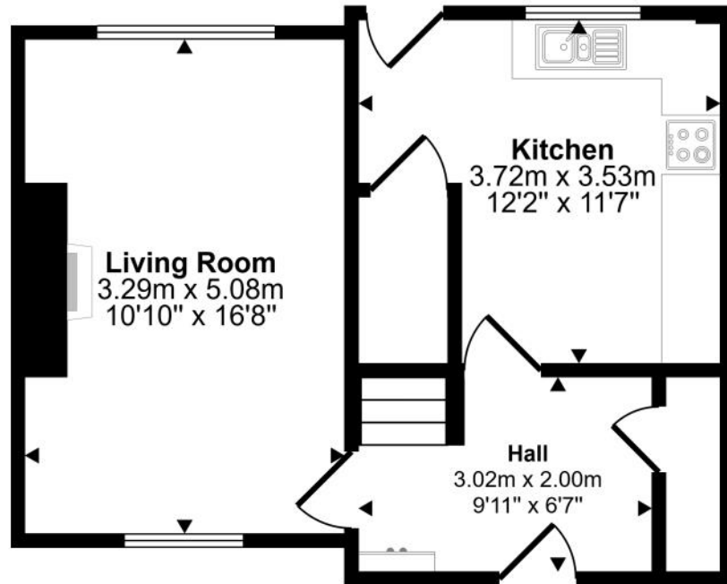
Ground Floor Approx 39 sq m / 415 sq ft
