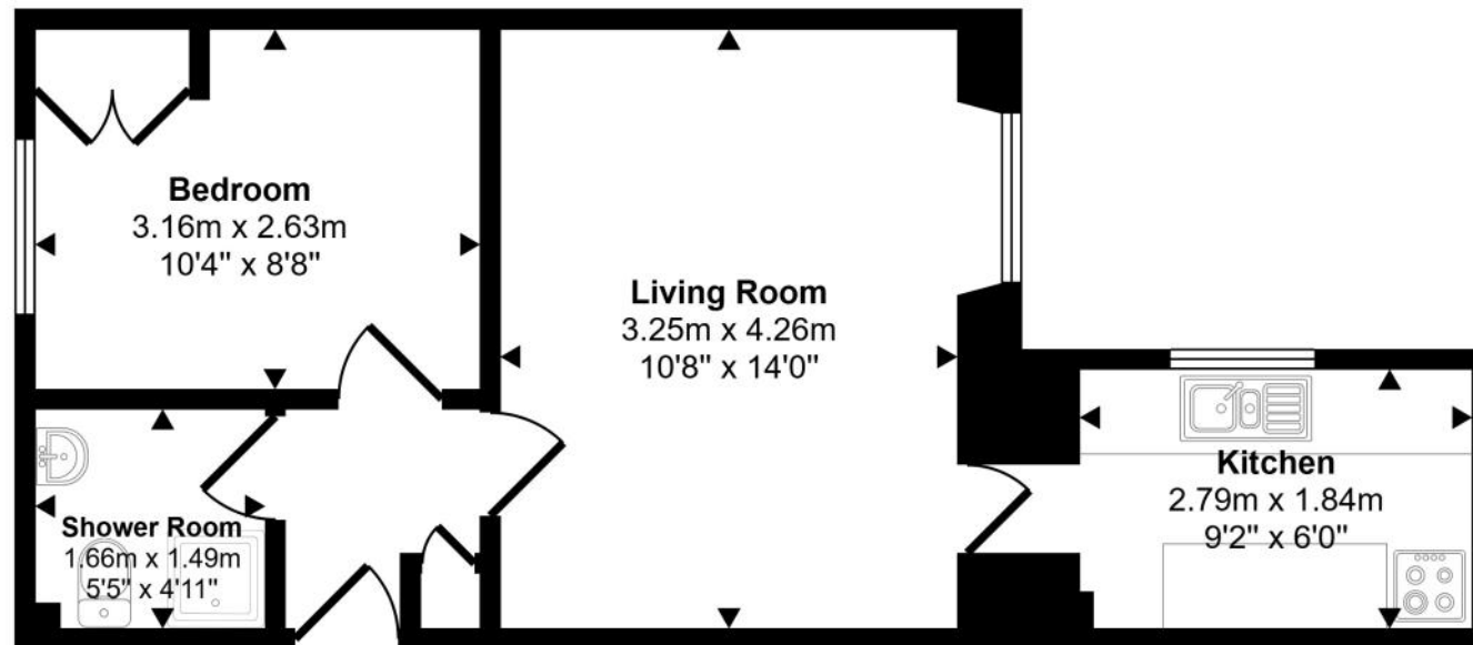
Floorplan
